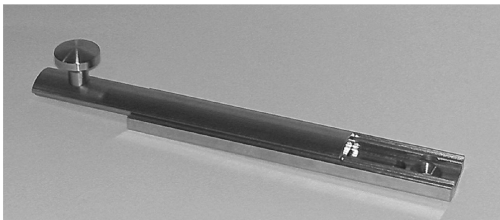
Photo 2: PA-31 Series Cabin Door Latch (Piper PN 472-004)
