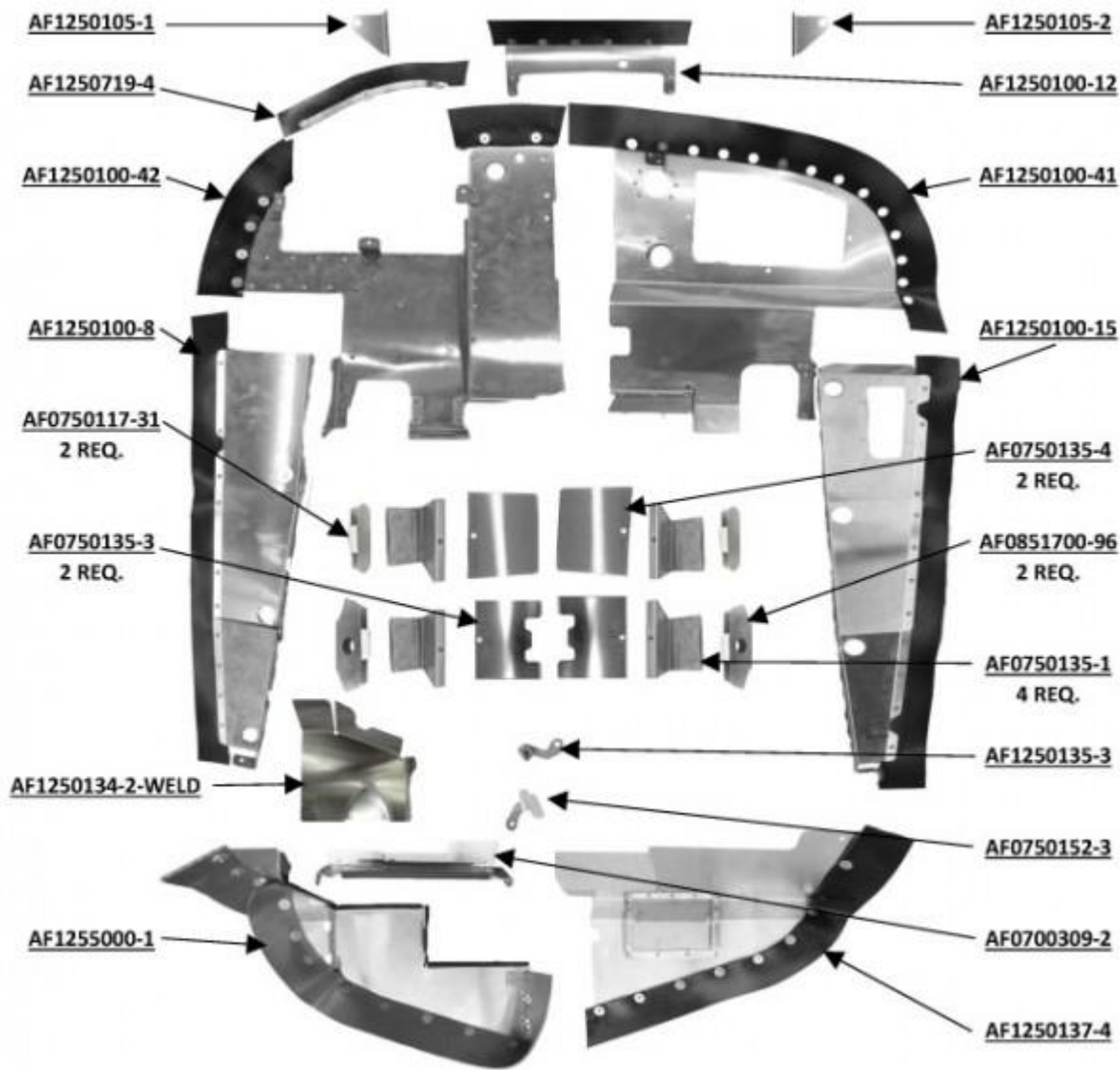
Photo 1: Airforms engine baffles for Cessna C210 – 1970-1973 aircraft
