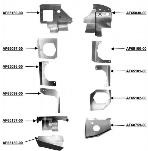
Photo 2: Airforms engine baffles for PA-28-235 Dakota aircraft
