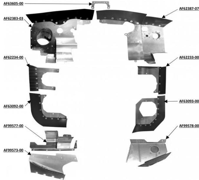
Photo 1: Airforms engine baffles for PA-28-180 1972.5 – 1975
