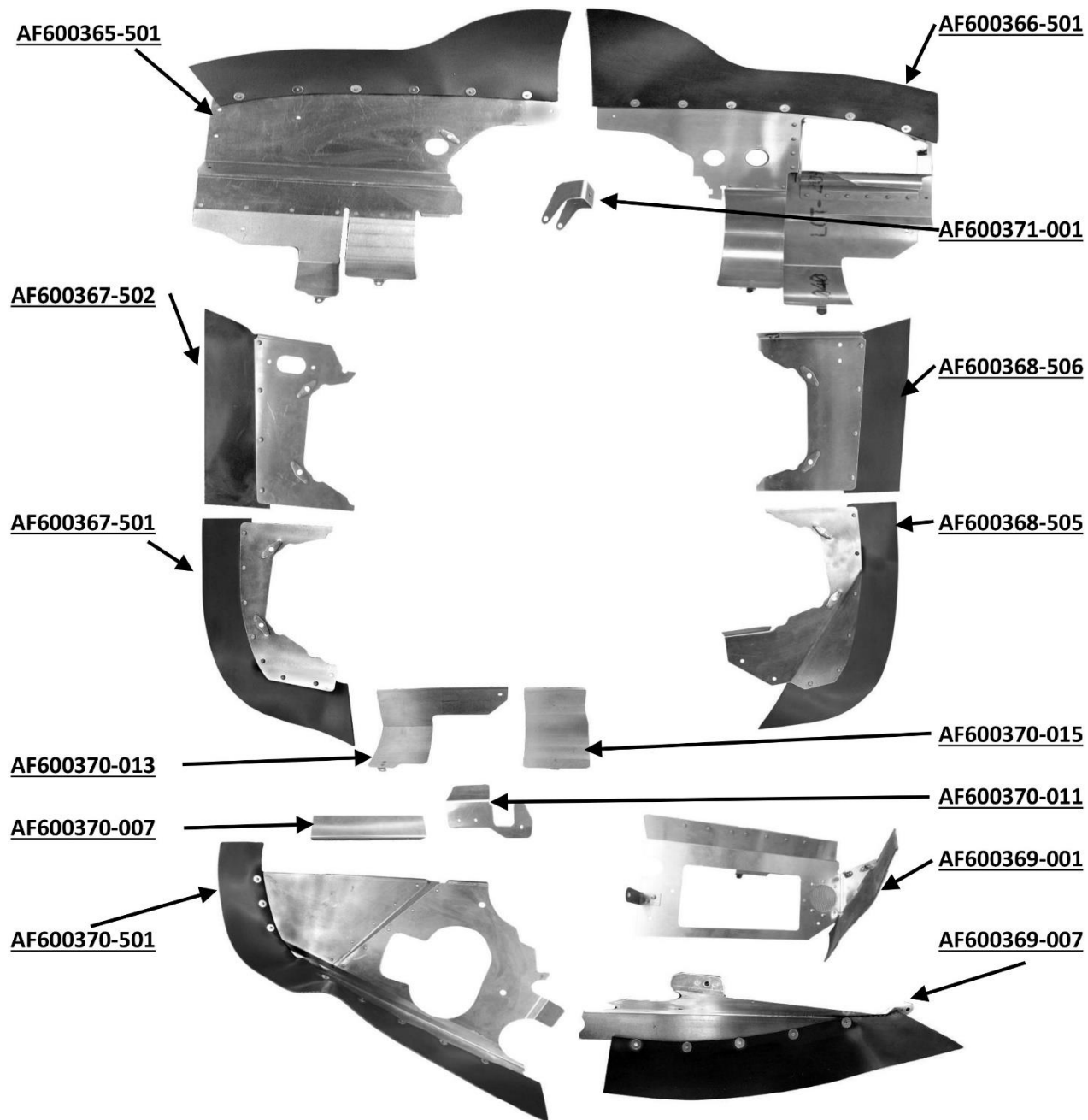
Photo 1: Airforms engine baffles for Mooney M20J aircraft
