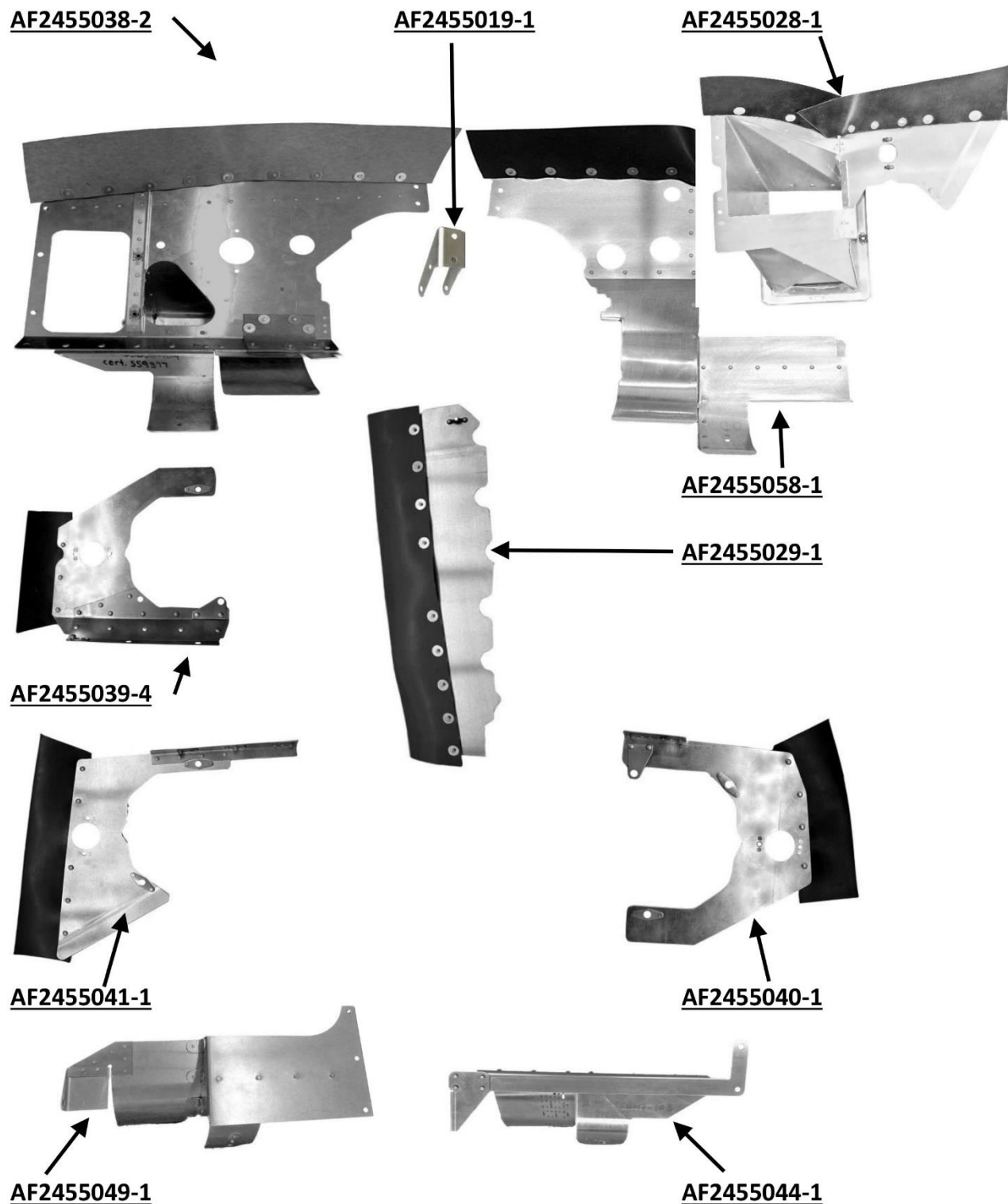
Photo 1: Airforms engine baffles for Cessna C172RG aircraft
