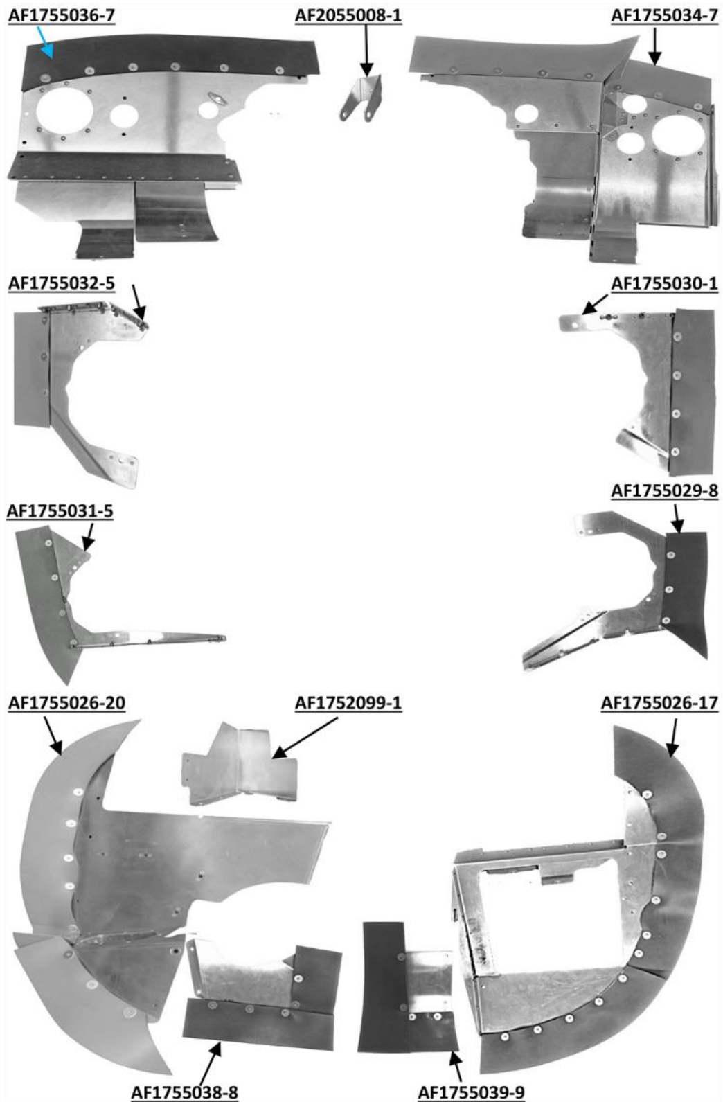
Photo 1: Airforms' engine baffles for 1973-1974 Cessna C177B
