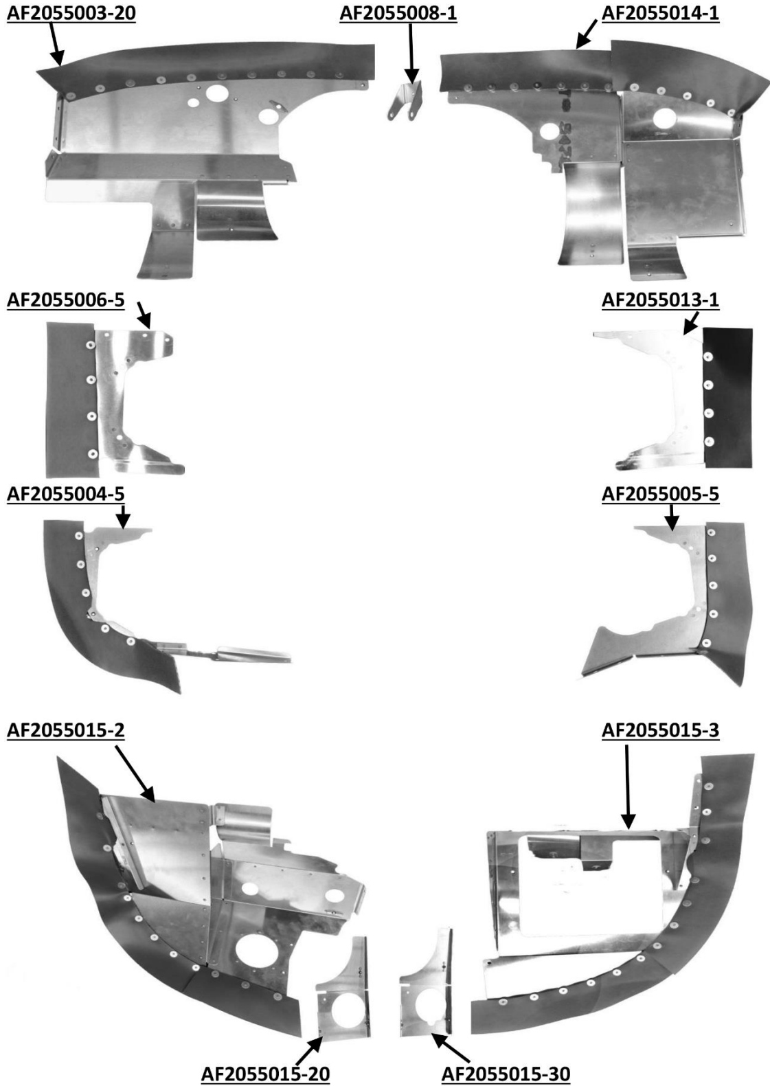
Photo 2: Airforms engine baffles for Cessna 177RGII
