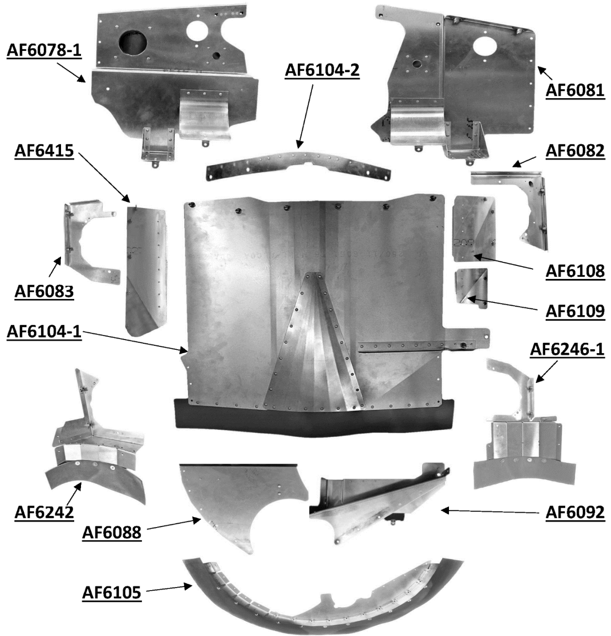
Photo 1: Airforms' engine baffles for Mooney M20B/C/D aircraft
