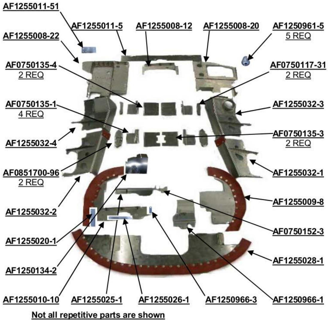
Photo 1: Airforms engine baffles for Cessna 210 (76-80) aircraft
